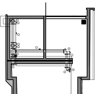
PREREZ 3-3 PRELIV IN IZPUST
