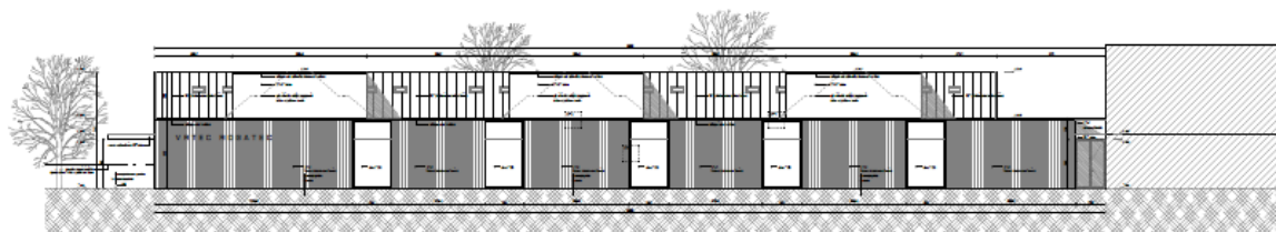
SEVERNA FAGADA
